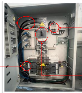
PV AC DB No.2 11SNPB-WAC01
