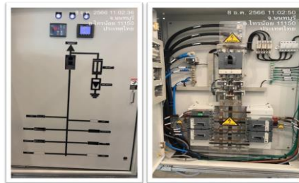
PV AC DB No.2 11SNPB-WAC01
